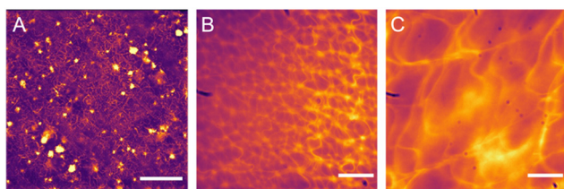
Fig. 15 Fluorescent microscopy images of self-associated fibres formed from (A) 4 , (B) 14 and (C) 36 (5 mg mL -1 ) in an aqueous solution of Na 2 SO 4 at 0.505 M. Scale bar A = 120 μm, B and C = 20 μm. Reproduced/adapted from ref. 5 with permission from RSC Journal of Material Chemistry B .
