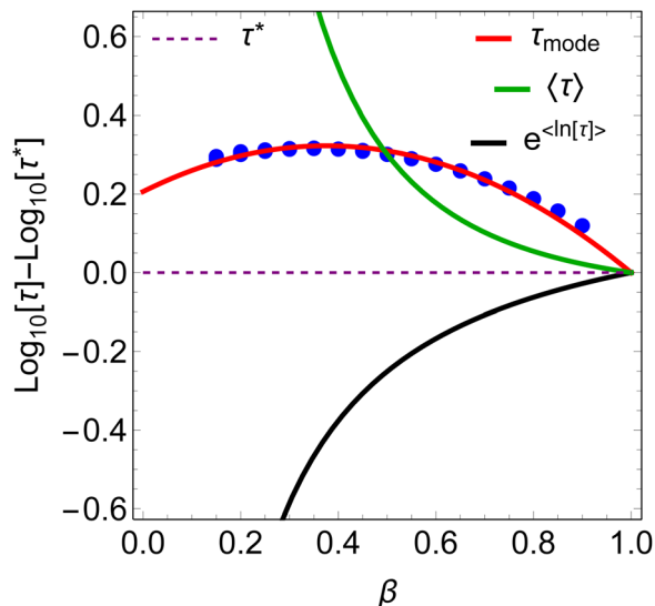
Fig. 4 \beta -Dependence of the four measures of \tau relative to \tau^* . Blue circles are the mode of the SEF distribution for -4 < \log[\tau^*] < 4 ; there is no observable dispersion.
