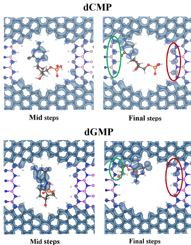
Fig. 5 Local density of states (LDOS) for G5BN in the presence of dCMP and dGMP.
