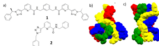
Fig. 1 (a) The chiral bis-tridentate (1,2,3-triazol-4-yl)-picolinamide (tzpa) ligand 1 used in the current study, and the ‘half’ ligand 2, which was formed as a model ligand. The solid state structures of the tetranuclear [2 × 2] square grids formed from 1 in our previous study using: (b) Cu(NO 3 ) 2 ·3 H 2 O and (c) [Cu(MeCN) 4 ](PF 6 ), respectively. 26
