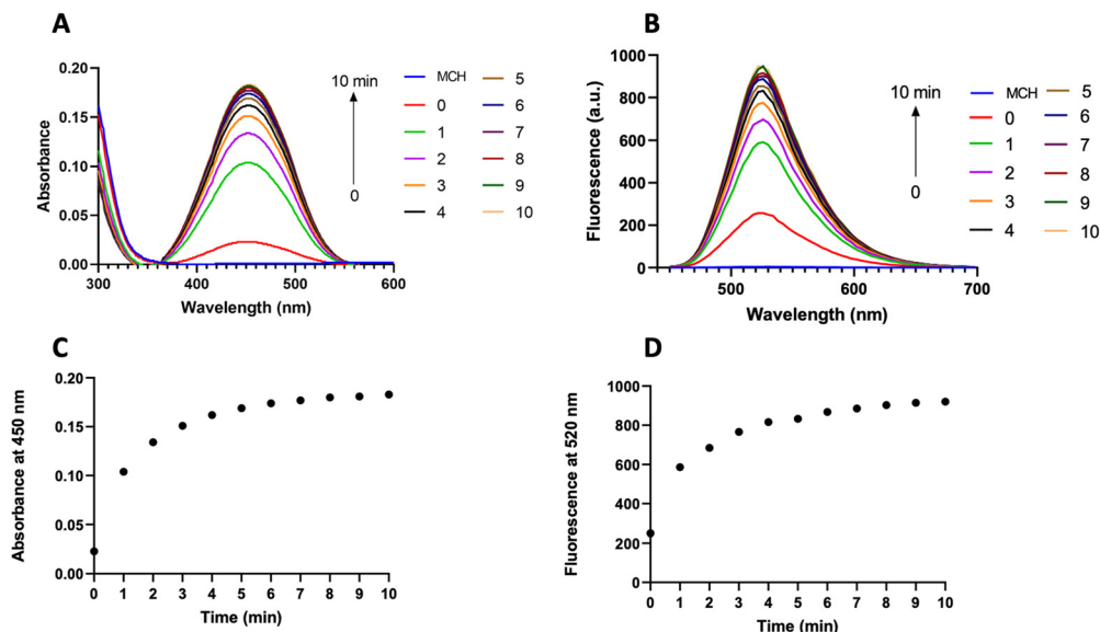
Fig. 2 (A) Absorption and (B) fluorescence spectra of MCH (10 \mu M) with or without the addition of 2 eq. of H 2 S in DMSO (2% PBS, pH 7.4) and (C) corresponding absorbance at 450 nm and (D) fluorescence at 520 nm in the presence of 2 eq. of H 2 S from 0 to 10 min. \lambda_{\text{ex}} = 440 nm.
