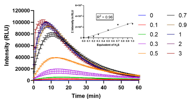
Fig. 3 Time-dependent chemiluminescence intensity of MCH (10 \mu M) in the presence of various equivalents of H 2 S (0–3) (inset: plot of the total luminescence with respect to varying H 2 S concentrations in the linear range) in DMSO (2% PBS, pH 7.4).
