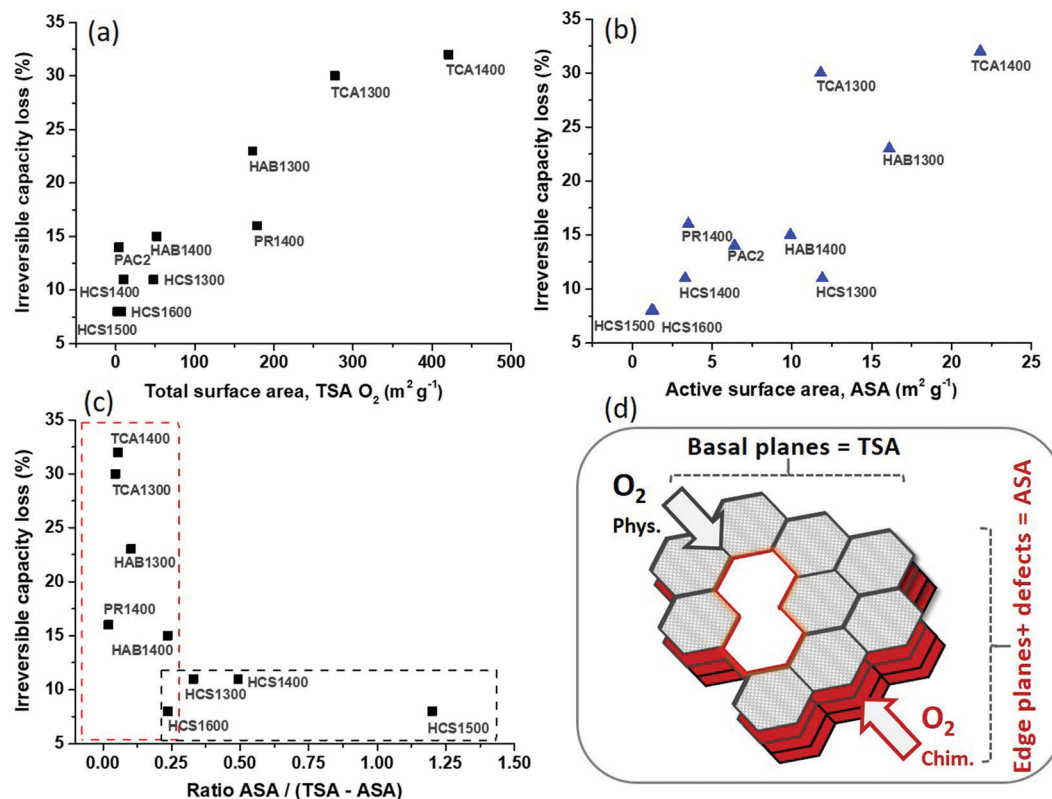
Fig. 3 Relationship between the 1st irreversible capacity loss and (a) total surface area ( TSA_{O_2} ), (b) active surface area ( ASA ), (c) ratio ASA/(TSA - ASA) . (d) Representation of hard carbon structure containing the active surface (edge planes and defects) and the basal planes surface ( TSA - ASA ).
