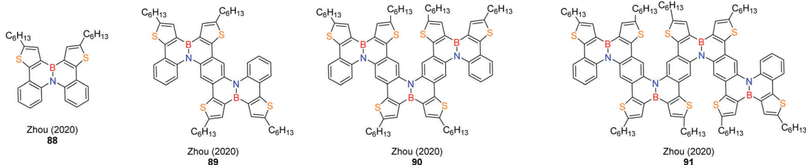
Fig. 26 BN-PAH oligomers with peripheral thiophenes.
