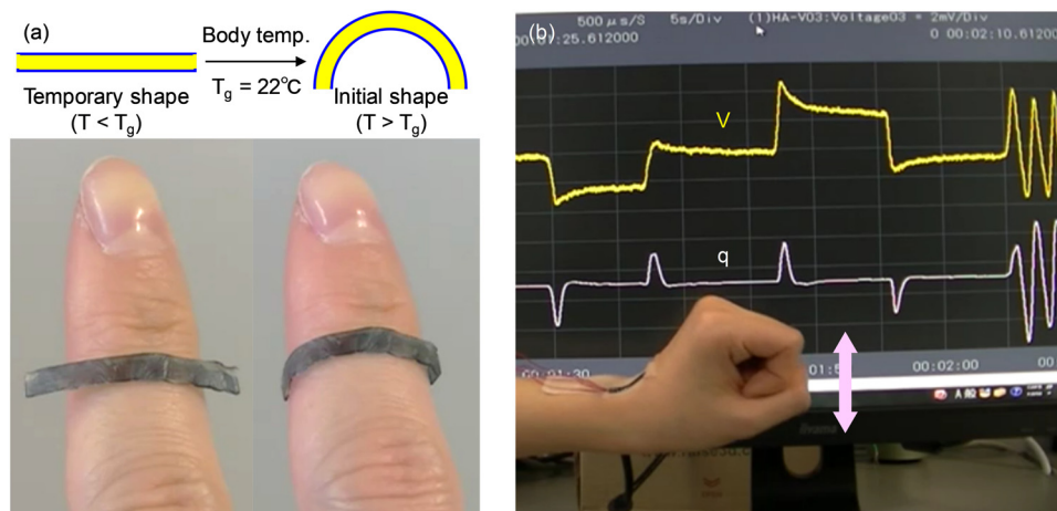
Fig. 9 (a) Schematic and photographs of ionic SMP gel sensor ( W_{IL} = 25 \text{ wt}\% ) with shape memory effect where temporary flat shape ( T < T_g ) recovers to initial curved shape on a finger at body temperature ( T > T_g ). (b) Photograph of a wearable sensor, fabricated with two equivalent ionic SMP gel sensors arranged in parallel by lamination with polyester films ( 100 \mu\text{m} thick), attached to the wrist detecting voltage ( V ) and charge ( q ) in response to shaking the wrist up and down.
