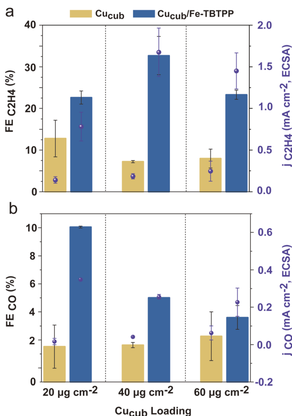
Fig. 7 (a) FE and partial current density for the C 2 H 4 product normalized by ECSA ( j_{\text{C}_2\text{H}_4/\text{ECSA}} ) and (b) FE and partial current density for the CO product normalized by ECSA ( j_{\text{CO}/\text{ECSA}} ) for Cu cub /Fe-TBTTP at different loading of Cu cub ( 3.12 \times 10^2 , 6.24 \times 10^2 and 9.36 \times 10^2 nmol cm -2 ) with the same Fe-TBTTP loading (16 nmol cm -2 ) at -0.95 V vs. RHE in the CO 2 saturated 0.1 M KHCO 3 H-cell. The reported values are an average of three independent experiments with error bars indicating the standard deviations.
