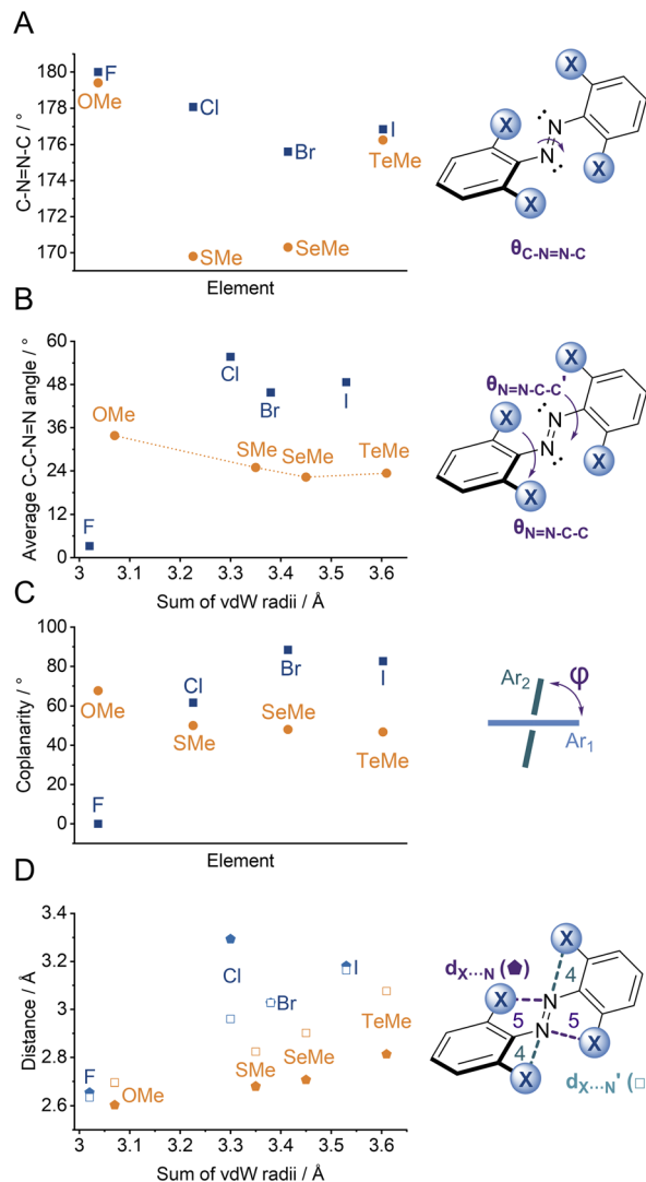
Fig. 5 Geometric parameters from single-crystal data for ( E )-X 4 C-N=N-C dihedral, (B) average N=N-C-C dihedral, (C) coplanarity of rings, (D) distances between diazo lone pair and X-atom (formation of intramolecular 5 (●) and 4 (□) membered rings).
