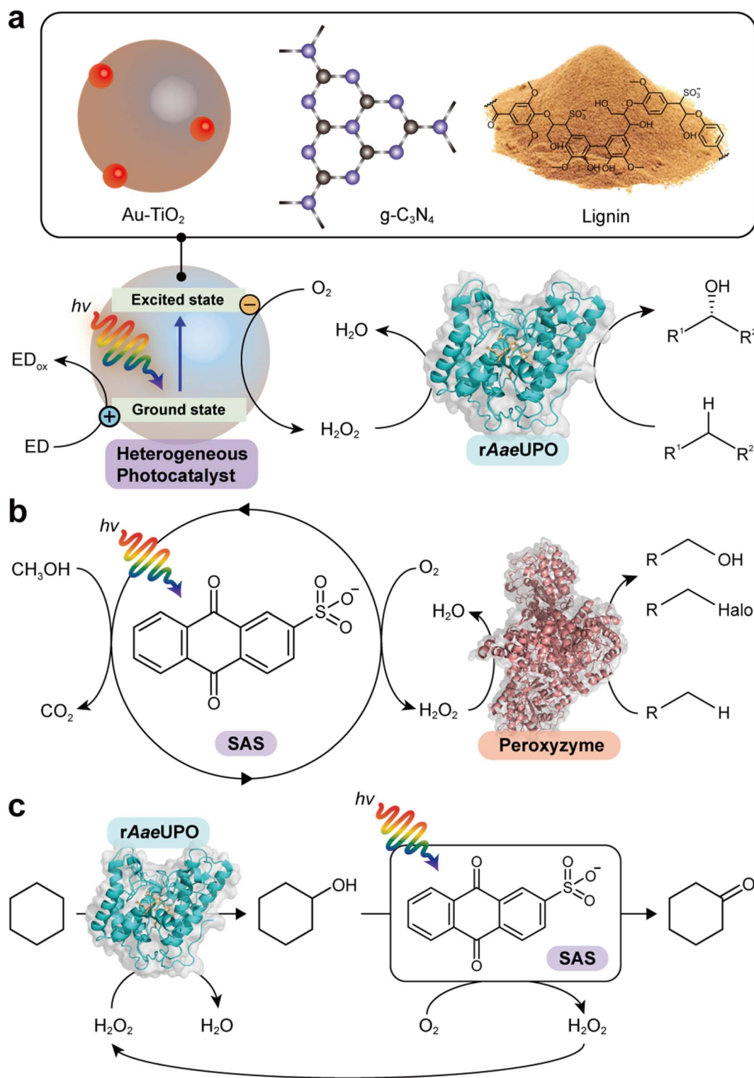
Fig. 6 Photocatalytic formation of \text{H}_2\text{O}_2 and selective oxidation reactions catalyzed by rAaeUPO and peroxylzyme. Representative photocatalysts include Au– \text{TiO}_2 , 90 g– \text{C}_3\text{N}_4 , 93 lignin 99 (a), and anthraquinone (SAS) 97,106 (b). (c) Photocatalytic oxidation of cyclohexane to cyclohexanone. The SAS-catalyzed aerobic overoxidation of cyclohexanol to cyclohexanone produces \text{H}_2\text{O}_2 as a byproduct, which itself is used to support the rAaeUPO-catalyzed hydroxylation of cyclohexane. 97
