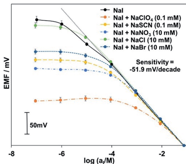
Fig. 35 Response of an ISE containing ionophore 30.XB toward iodide in the absence of presence of competing anions. Reproduced with permission from ref. 166 copyright 2021 American Chemical Society.
