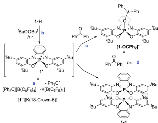
Scheme 4 Generation of 1' , its dimerization and trap with benzophenone.
