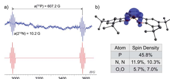
Fig. 5 (a) EPR spectra of 1' (blue) and its simulation (red); (b) DFT calculated structure and Mulliken spin densities of 1' .
