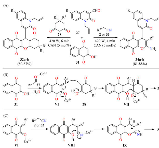
Scheme 7 (A) CAN-catalyzed three-component synthesis of N -allylquinolone derivatives 32 and 34 and their in vitro antibacterial activity against four bacterial strains. (B) Plausible reaction mechanism for the formation of 32 . (C) Plausible reaction mechanism for the formation of 34 .
