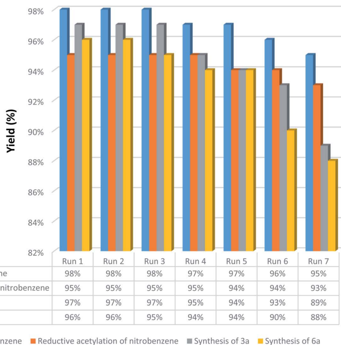
Fig. 11 Recoverability and reusability experiments of the dendritic \text{Fe}_3\text{O}_4@ \text{SiO}_2@ \text{KCC-1@MPTMS@Cu}^{\text{II}} mesoporous nanocomposite.
