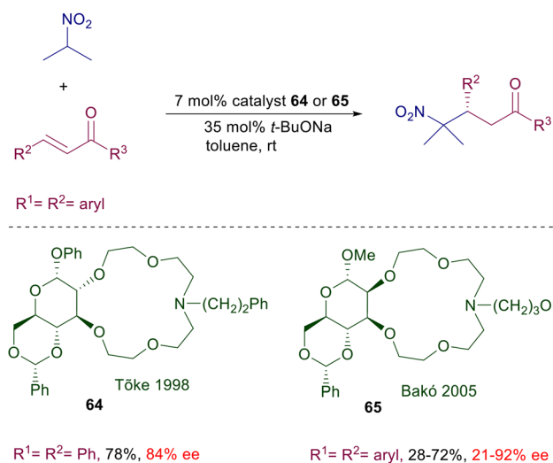
Scheme 48 Monoaza-15-crown-5 ethers as phase transfer catalysts.
