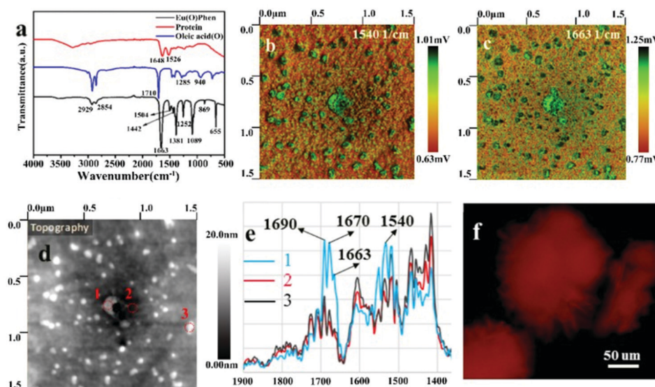
Fig. 11 The concentration of oleic acid used during nano-label synthesis was 0.05 \text{ mol L}^{-1} in FTIR spectra and PiFM images. (a) FTIR spectra of protein, oleic acid, and OEu 3+ Phen complexes; PiFM images taken with laser tuned to (b) 1540 \text{ cm}^{-1} for protein and (c) 1663 \text{ cm}^{-1} for OEu 3+ Phen complexes in the sample; (d) the detection points of the sample, overlaid on a topographical map; (e) PiFM infrared spectra for the detection points; (f) the fluorescence microscopy image of the sample. Reproduced from Zhao et al. 61
