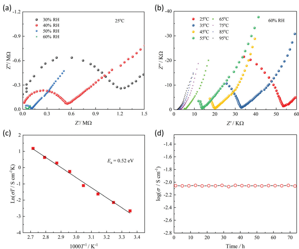
Fig. 2 (a) Impedance spectra of 2 under 30–60% RH at RT. (b) The variable temperature impedance spectra of 2 from 25 to 95 °C at 60% RH. (c) Arrhenius plot. (d) Time-dependent proton conductivity of 2 at 95 °C and 60% RH.
