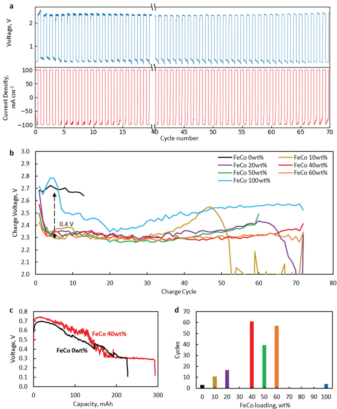
Fig. 8 (a) A typical charge/discharge profile of a ZAB using FeCo rGO 40 wt% at 100 \text{ mA cm}^{-2} . (b) Charging potential at the end of every charging cycle for FeCo 0 wt% (black), FeCo 10 wt% (brown), FeCo 20 wt% (purple), FeCo 40 wt% (red), FeCo 50 wt% (green), FeCo 60 wt% (orange), and FeCo 100 wt% (blue). Charging potential decreased by 0.4 V between FeCo 0 wt% (black) and FeCo 10–60 wt% (c) Discharge profiles of a ZAB with FeCo 0 wt% and FeCo 40 wt%. (d) Average number of cycles at 100 \text{ mA cm}^{-2} before the discharge capacity decreases below 90% with FeCo of various loading levels.
