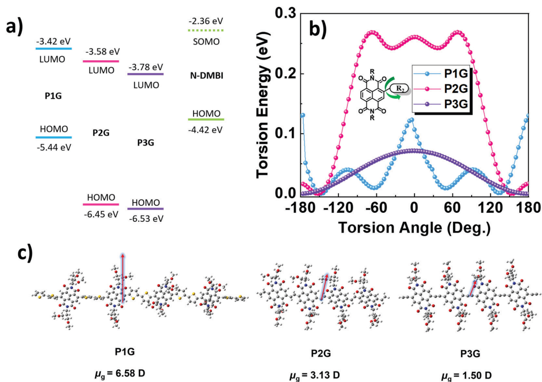
Fig. 1 Results from DFT calculations. (a) energy levels of CPs and N-DMBI (b) torsion energy profiles of the NDI- R_2 bond. (c) Energy minimized 3D structure and dipole moments of the backbone of tetramer models for CPs, arrows are vectors depicting the magnitude and direction of the dipole moment.
