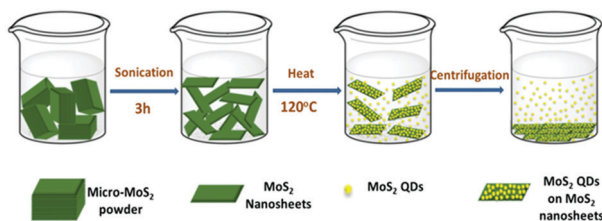
Fig. 16 Illustration of reaction steps for sonochemical synthesis of MoS 2 QDs and nanosheets. Reprinted with permission from ref. 110 [S. Xu, D. Li and P. Wu, Adv. Funct. Mater. , 2015, 25 , 1127–1136]. Copyright WILEY-VCH Verlag GmbH & Co. KGaA, Weinheim.
