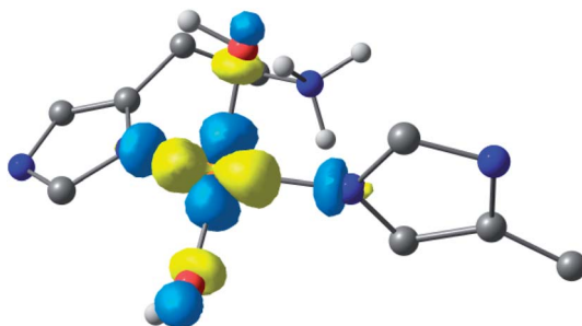
Fig. 6 Hypothetical d(x^2 - y^2) dominated SOMO of species 2 showing that the orbital plane has rotated (the colours denote the orbital phases).
