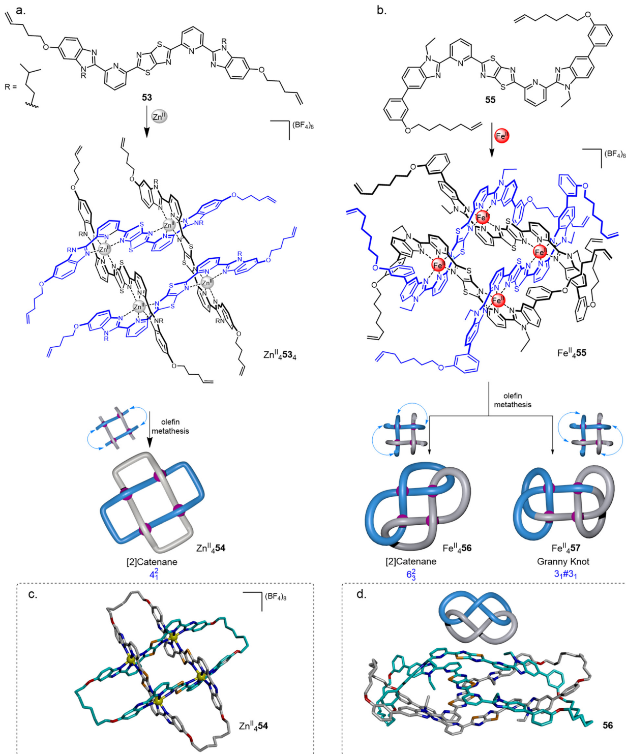
Fig. 20 Synthesis of 2 × 2 interwoven molecular grids and their closures by olefin metathesis to generate (a) Solomon link 54 , 14 or (b) 6 2 link 56 and granny knot 57 , 15 X-ray crystal structures of (c) Zn II 4 54 and (d) demetallated link 56 .
