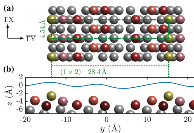
Fig. 1 (a) Top view of the (1 × 2) reconstructed Bi(114) surface. (b) Side view of the atomic structure of Bi(114) surface along the \overline{\Gamma Y} -direction, illustrating the asymmetry upon scattering normal to the steps. An exemplary corrugation function (eqn (3)) using j = 3 terms with h = [0.435, 0.43, 0.14] and \alpha = \left[-\frac{\pi}{2}, \frac{\pi}{2}, \frac{\pi}{2}\right] is drawn as solid blue line above the side view of the atomic structure.
