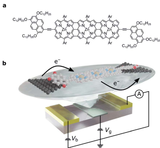
Fig. 1 (a) The molecular structure of FP3 : the edge-fused porphyrin trimer core is functionalized in the terminal meso positions by trido-decyloxyphenyl groups for anchoring to graphene source and drain electrodes. Ar groups are solubilizing aryl groups, 3,5-bis(trihexylsilyl) phenyl. (b) Device architecture: nanometer-separated graphene source and drain electrodes are electroburnt from a graphene ribbon between two gold electrodes. The graphene is patterned into a bowtie shape, and a local gate electrode separated from the molecule by a thin layer of \text{HfO}_2 (grey) is used to shift the molecular energy levels. For clarity, the bulky side-groups are omitted.
