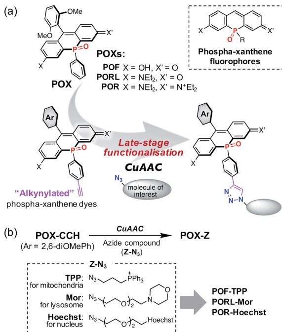
Fig. 1 (a) Functionalisation of phospho-xanthenes fluorophores shown in a dashed box. A phenyl ring on the phosphorus atom of the parent POX dyes is modified with an ethynyl group. The alkylnated phospho-xanthenes dyes thus obtained can be converted into the corresponding triazole compounds via a copper-catalysed azide–alkyne cycloaddition (CuAAC) at the late stage of synthesis. (b) POX-based organelle markers obtained from alkylnated-POXs (POX-CCHs) and azide compounds used in this work.
