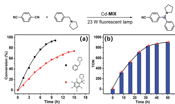
Fig. 4 (a) Kinetics curves of the C–H arylation using N -benzylpyrrolidine or N -((phenyl- D_5 )methyl- D_2 )pyrrolidine with 1,4-dicyanobenzene under optimal conditions. (b) The turnover number in scale-up experiments for C–H arylation of N -benzylpyrrolidine with 1,4-dicyanobenzene (0.64 g) within 50 h under optimal conditions.
