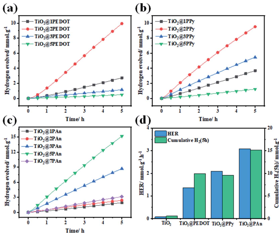
Fig. 10 Time course of \text{H}_2 evolution over 50 mg of different weight percent of (a) poly(3,4-ethylenedioxythiophene) (b) polypyrrole (c) polyaniline relative to \text{TiO}_2 (P25) in a 20% vol. aqueous methanol under UV light irradiation for 5 h (d) Histograms of optimum samples.
