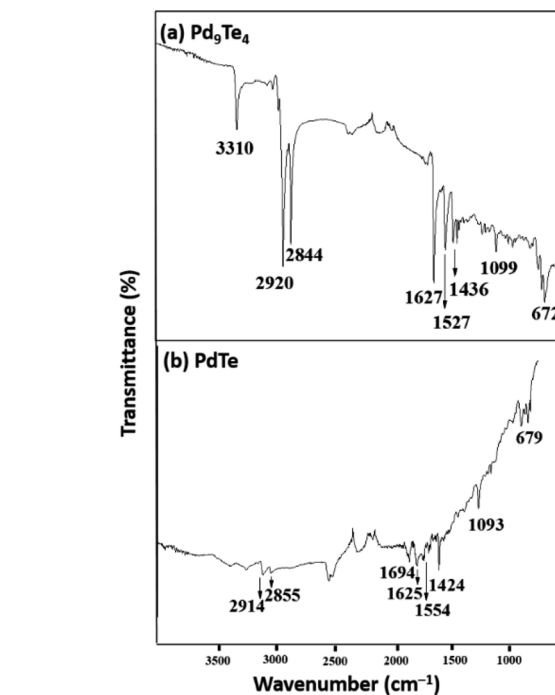
Fig. 4 FTIR spectra of (a) Pd 9 Te 4 (b) PdTe nanostructures.
