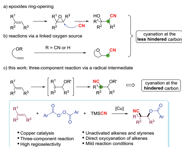
Scheme 1 Oxyanation of alkenes.
