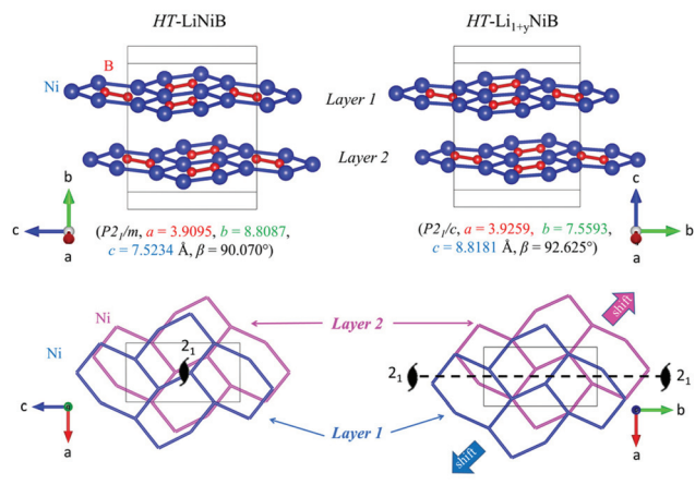
Fig. 5 Comparison between [NiB] layers in the structures of HT\text{-LiNiB} and HT\text{-Li}_{1+y}\text{NiB} compounds. The lower panel shows a relative shift between two adjacent [NiB] layers in the structures of HT\text{-LiNiB} and HT\text{-Li}_{1+y}\text{NiB} .
