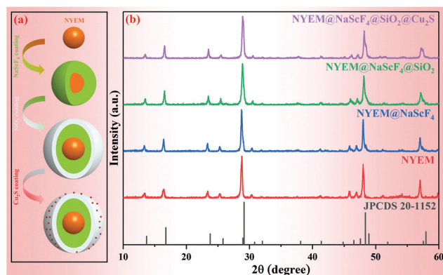
Fig. 1 (a) A description of the preparation of \text{NYEM}@(\text{NaScF}_4)_n@(\text{SiO}_2)_m@(\text{Cu}_2\text{S})_p . (b) XRD diffraction patterns of the samples synthesized at various steps along with the reference data of hexagonal \text{NaScF}_4 (JCPDS 20-1152).
