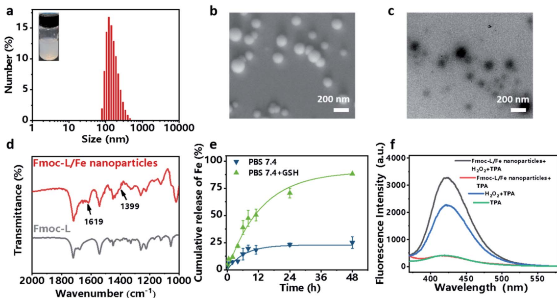
Fig. 2 (a) DLS profile with a digital picture and (b) SEM image and (c) TEM image of the as-prepared Fmoc-L/Fe nanoparticles. (d) FTIR spectra of Fmoc-L/Fe and Fmoc-L. (e) GSH-responsive release profile of \text{Fe}^{2+} from Fmoc-L/Fe nanoparticles. (f) The change of fluorescence emission spectra of TPA after treatment with Fmoc-L/Fe nanoparticles with or without \text{H}_2\text{O}_2 .
