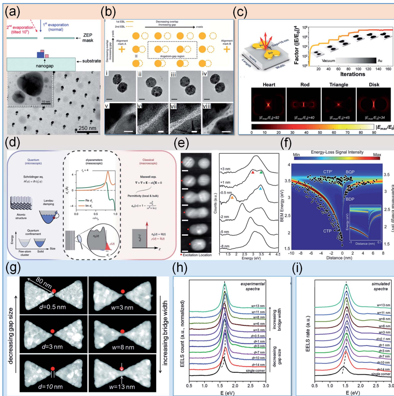
Fig. 9 (a) Schematic diagram of the angle evaporation technique and the SEM of obtained nanostructures. 126 (b) Schematic depiction of the two-step EBL process and the TEM images of four representative dimers. 127 (c) The 3D model and the electric-field distribution of heart-, rod-, triangle-, and disk-shaped Au nanoparticle dimers. 102 (d) Nonclassical mesoscopic electrodynamic theory via d -parameters. 141 (e) STEM images correlated with experimental plasmonic spectra and theoretical field profiles of a merging dimer. (f) Comparison of classical BEM EELS calculations with experimental EELS resonances. 123 (g–i) Representative HAADF STEM images of the experimental samples with different junction geometries (g), experimental EELS spectra (h) and simulated spectra (i) of the dark modes of structures 136 (reproduced with permission from ref. 102 Copyright 2020 Wiley-VCH, ref. 123 Copyright 2013, ref. 126 Copyright 2010 and ref. 136 Copyright 2012 the American Chemical Society, ref. 127 Copyright 2014, Nature Publishing Group, ref. 141 Copyright 2020, the Authors).
