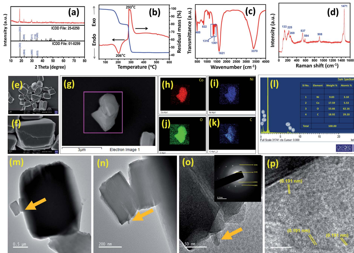
Fig. 1 (a) PXRD with the standard patterns of \text{Ni}_2\text{O}_4 \cdot 2\text{H}_2\text{O} (ICDD no. 01-0299) and \text{Co}_2\text{O}_4 \cdot 2\text{H}_2\text{O} (ICDD no. 25-0250), (b) DTA-TG, (c) FTIR and (d) Raman pattern of the as-prepared nickel-cobalt oxalate ( \text{Ni}_{2.5}\text{Co}_5\text{C}_2\text{O}_4 ) sample. Morphological study including (e and f) FESEM images, (g–k) elemental mapping, (l) EDS study, (m–o) TEM images (the inset showing SAED) and (p) HRTEM image of the as-prepared nickel-cobalt oxalate ( \text{Ni}_{2.5}\text{Co}_5\text{C}_2\text{O}_4 ) sample.
