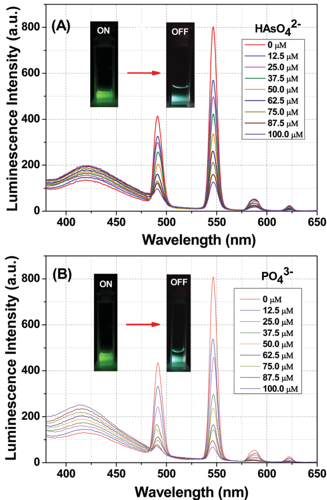
Fig. 4 (A) Emission spectra of 1a dispersed in aqueous solution upon the incremental addition of an aqueous solution of \text{HAsO}_4^{2-} ions ( \lambda_{\text{ex}} = 280 nm). The final concentration of \text{HAsO}_4^{2-} ions in the medium is indicated in the legend. (B) Emission spectra of 1a dispersed in an aqueous solution upon the incremental addition of an aqueous solution of \text{PO}_4^{3-} ions ( \lambda_{\text{ex}} = 280 nm). The final concentration of \text{PO}_4^{3-} ions in the medium is indicated in the legend. The inset figure in both cases shows the colour change of green emission of 1a after the incorporation of \text{HAsO}_4^{2-} and \text{PO}_4^{3-} anions.
