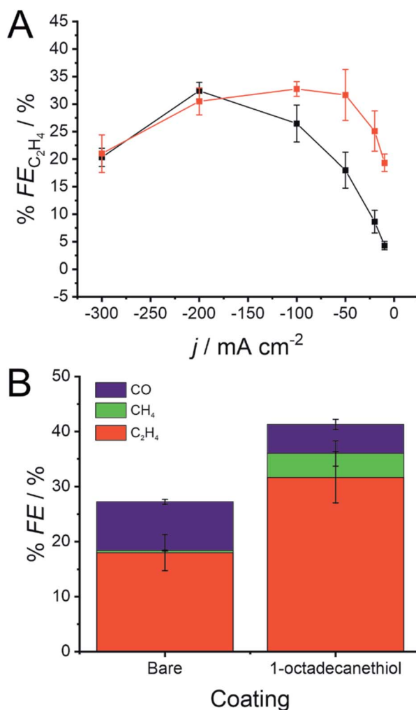
Fig. 4 (A) Faradaic efficiency for \text{C}_2\text{H}_4 formation ( \% \text{FE}_{\text{C}_2\text{H}_4} ) during galvanostatic \text{CO}_2 reduction at a 500 nm Cu GDE in 1 M KOH with (red) and without (black) a monolayer of 1-octadecanethiol to form a hydrophobic interface. (B) % FE for CO, \text{CH}_4 and \text{C}_2\text{H}_4 with and without the 1-octadecanethiol layer during galvanostatic \text{CO}_2 reduction at -50 \text{ mA cm}^{-2} using the same conditions as in (A). Error bars display one standard deviation ( n = 3 ).
