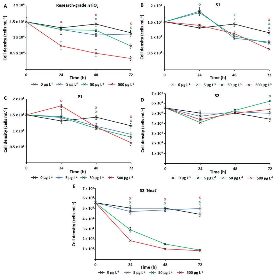
Fig. 2 Cell density of Prochlorococcus MED4 when exposed to nTiO 2 (0–500 μg L -1 ) for a period of 72 h under simulated natural conditions as measured by flow cytometry; A – research-grade nTiO 2 nanopowder purchased from Sigma Aldrich; B – nTiO 2 extracted from SkinCeuticals™ sunscreen (S1); C – nTiO 2 extracted from The Body Shop™ liquid foundation (P1); D – nTiO 2 extracted from Boots Soltan™ sunscreen (S2); E – ‘Neat’ Boots Soltan™ sunscreen immersed in NSW. Data points are presented as the mean ± standard error ( n = 3 ). Markers indicate where two-way t -tests revealed cell density of treated groups to be significantly lower (crosses) or higher (circles) than the untreated control at each timepoint ( p \leq 0.05 ).
