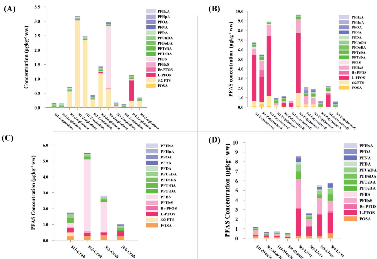
Fig. 3 Average concentration of PFAS ( \mu\text{g kg}^{-1} ww) detected in biota samples in the vicinity of Longyearbyen (Svalbard); (A) zooplankton; (B) polychaetes; (C) local crab samples (standard error of the mean is given in Table S17†); (D) local fish samples (muscle and liver) collected in the vicinity of Longyearbyen (Svalbard, standard error of the mean is given in Tables S19 and S20†).
