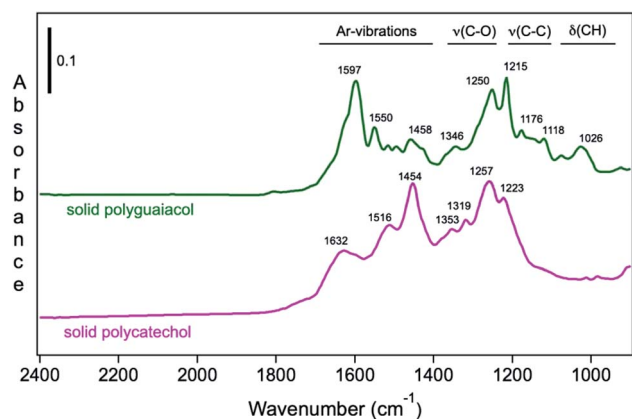
Fig. 9 ATR-FTIR absorbance spectra of (a) solid polyguaiacol (top) and polycatechol (bottom) deposited on a ZnSe ATR crystal from a water/ethanol slurry, followed by drying overnight. Reproduced from ref. 70 with permission from the American Chemical Society, © 2015.
