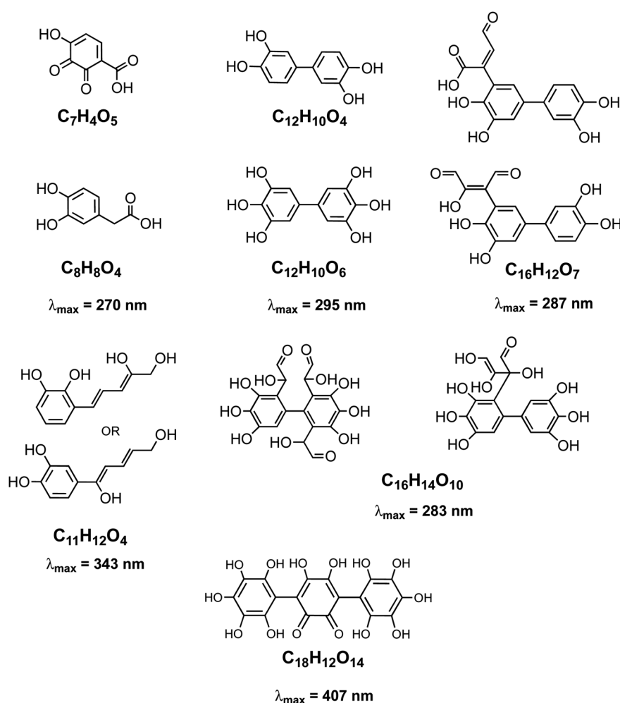
Scheme 2 Structure of molecules and oligomers and their characteristic absorption wavelength detected in the reaction of catechol with \text{Fe(III)} under conditions characteristic of viscous multicomponent aerosol systems with relatively high ionic strength ( I = 1\text{--}12 \text{ m} ) and acidic pH ( \sim 2 ) using UHPLC-MS. Modified from ref. 148 with permission from The American Chemical Society, © 2021.
