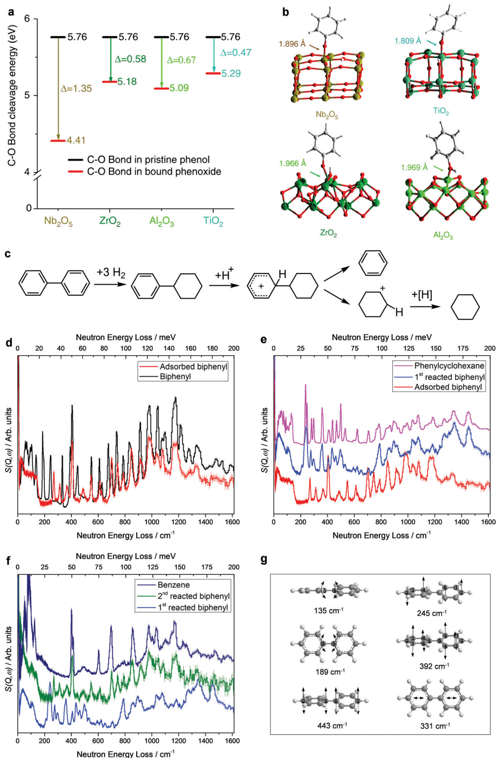
Fig. 3 Conversion of lignin to aromatics. (a) Calculated energies for dissociation of the C–O bonds of phenol upon adsorption over Nb 2 O 5 , ZrO 2 , Al 2 O 3 and TiO 2 . (b) Views of the corresponding DFT-optimised structural models for phenoxide bound on the Nb 2 O 5 (001), ZrO 2 (010), Al 2 O 3 (110) and TiO 2 (101) surfaces. Adapted from ref. 34 published by Springer Nature, licensed under a Creative Commons Attribution 4.0 International License ( https://creativecommons.org/licenses/by/4.0/legalcode ). (c) Possible reaction mechanism in the conversion of biphenyl over the Ru/NbOPO 4 catalyst. Inelastic neutron scattering (INS) spectra for Ru/NbOPO 4 in the adsorption and catalytic conversion of biphenyl. All spectra shown here are difference spectra. (d) Comparison of INS spectra for solid and adsorbed biphenyl on Ru/NbOPO 4 . INS spectra for Ru/NbOPO 4 during the first (e) and second (f) catalytic conversion of biphenyl. (g) Views of selected C–C vibration modes of biphenyl. Reproduced with permission from ref. 35, Copyright © 2019 Elsevier.
