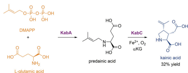
Scheme 12 Enzymatic total synthesis of kainic acid. KabA: N -prenyltransferase; KabC: \alpha -ketoglutarate-dependent dioxygenase; \alpha\text{KG} : \alpha -ketoglutarate. Starting materials are highlighted in orange. The product is highlighted in blue. Key enzymes in this synthetic route are highlighted in purple.
