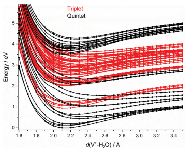
Fig. 2 Splined potential energy surface scans for the relevant quintet and triplet states along the water dissociation coordinate d(V^+-(H_2O)) on the CASSCF(4,9)/aug-cc-pVDZ level of theory, respectively. All other internal coordinates are kept at the values calculated for the minimum.
