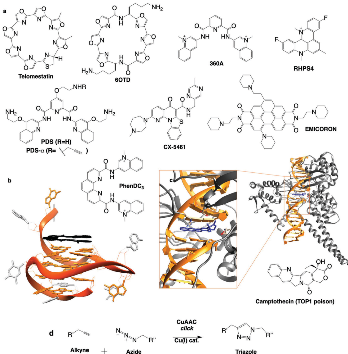
Fig. 7 (a) Chemical structures of G4 ligands. (b) NMR structure of G4 with PhenDC3 ligand (PDB ID: 2MGN). 263 (c) Crystal structure of TOP1cc with camptothecin (PDB ID: 1T8I). 311 (d) Bioorthogonal copper catalysed click ligation performed in cells between PDS \alpha and an azide-labelled fluorophore.
