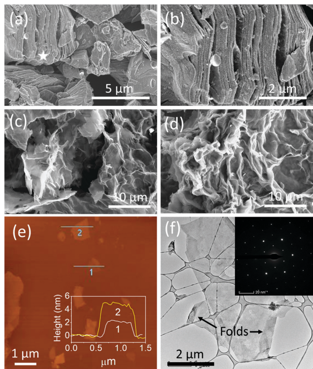
Fig. 2 (a) and (b) SEM micrographs of Ti_3C_2T_x after HF-etching of Ti_3AlC_2 MAX phase, (c) and (d) SEM micrographs of Ti_3C_2T_x and r-Ti_3C_2T_x powders, respectively, (e) Tapping mode AFM image of Ti_3C_2T_x nanosheets on SiO_2/Si , and (f) high magnification TEM image of a Ti_3C_2T_x nanosheet suspended over a holey carbon grid. The inset shows the selected area electron diffraction (SAED) pattern.
