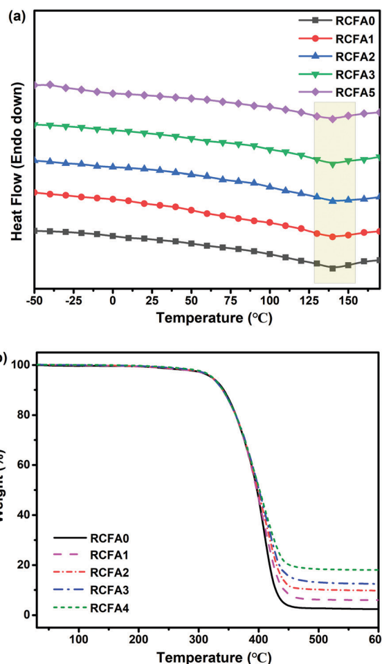
Fig. 4 (a) DSC curves of RCFA with different modified MWCNT contents. (b) TGA curves of RCFA with different modified MWCNT contents.
