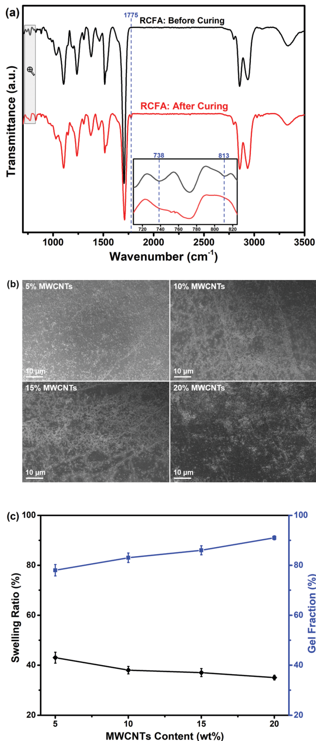
Fig. 3 (a) FTIR spectra of RCFA before and after curing. (b) SEM images of RCFA with different contents of modified MWCNTs. (c) Swelling ratio and gel fraction of RCFA with different modified MWCNT content.
