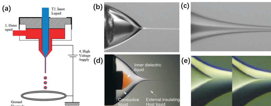
Fig. 14 (a) Schematic of a typical experimental setup for coaxial electrospinning. Reproduced with permission from ref. 6. Copyright 2002, The American Association for the Advancement of Science. 6 The structure of a coaxial compound Taylor-cone and its cone-jet (b and c) in air. Reproduced with permission from ref. 6. Copyright 2002, The American Association for the Advancement of Science. 6 (d and e) In insulating liquids, the meniscus of the inner liquid emits a jet as its flow rate increases. Reproduced with permission from ref. 176. Copyright 2007, American Physical Society. 176
