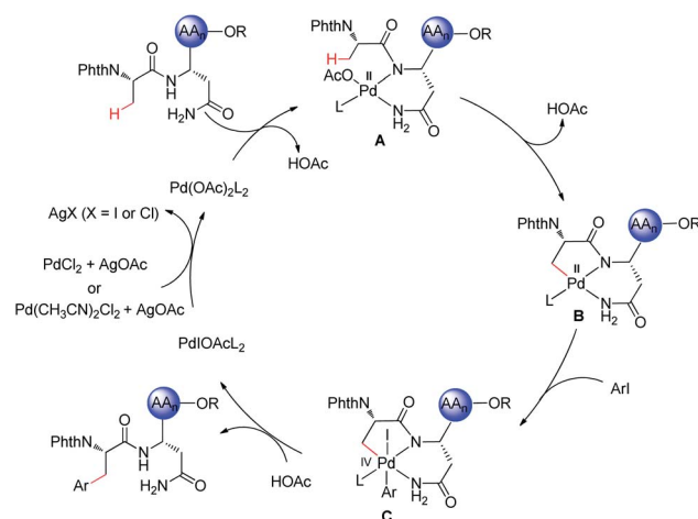
Scheme 4 Proposed mechanism.
