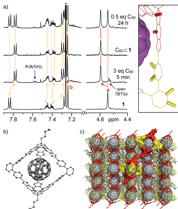
Fig. 3 (a) 1 H-NMR spectra (400 MHz, CDCl 3 , rt) for complexation of 1 with C 60 , (b) ORTEP representation of single-crystal X-ray structure of C 60 C1 (thermal ellipsoids were set at 50% probability, C = grey, O = red, B = purple, H atoms were omitted for clarity) and (c) packing of C 60 C1 in the solid state indicating the accessible C 60 surface in the three cage windows.
