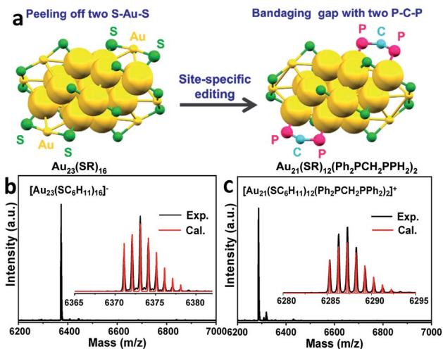
Fig. 3 (a) A schematic diagram of the site-specific editing of \text{Au}_{23}(\text{SR})_{16} by resecting two RS–Au–SR motifs and bandaging the gaps with two \text{Ph}_2\text{P–CH}_2\text{–PPh}_2 staples to obtain \text{Au}_{21}(\text{SR})_{12}(\text{Ph}_2\text{PCH}_2\text{PPh}_2)_2 . Color codes: yellow = Au; green = S; pink = P; blue = C. Carbon tails are omitted for clarity. SR = cyclohexanethiol. The ESI-MS spectra of (b) [\text{Au}_{23}(\text{SC}_6\text{H}_{11})_{16}]^- and (c) [\text{Au}_{21}(\text{SC}_6\text{H}_{11})_{12}(\text{Ph}_2\text{PCH}_2\text{PPh}_2)_2]^+ .
